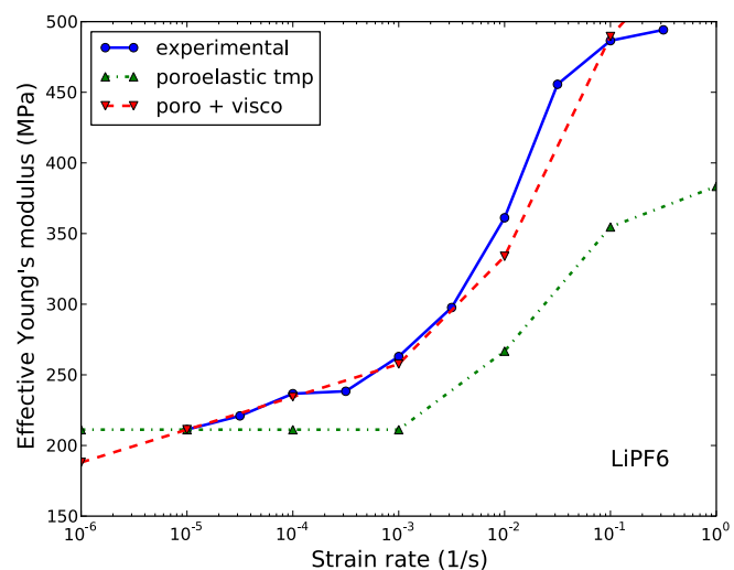
Figure 11. Effective Young's modulus of the separator immersed in 1 M LiPF 6 solution in EC/DMC as a function of strain rate. Solid line represents the experimental data from, 14 dash-dot line shows the results of calculations based on linear poroelastic behavior of the dry separator; red line shows the results of calculations, which take into account viscoelastic behavior of the dry separator and softening of the separator in solution when solving the equations of poroelasticity.
