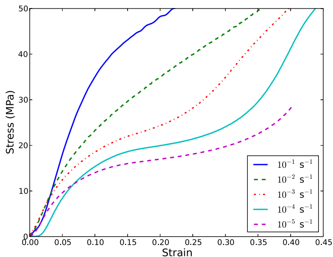
Figure 5. Experimental stress-strain curves for the separator immersed in water.
