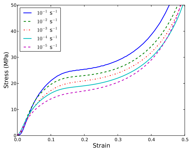
Figure 3. Stress-strain curves for the compression of the dry separator at constant strain rates.
