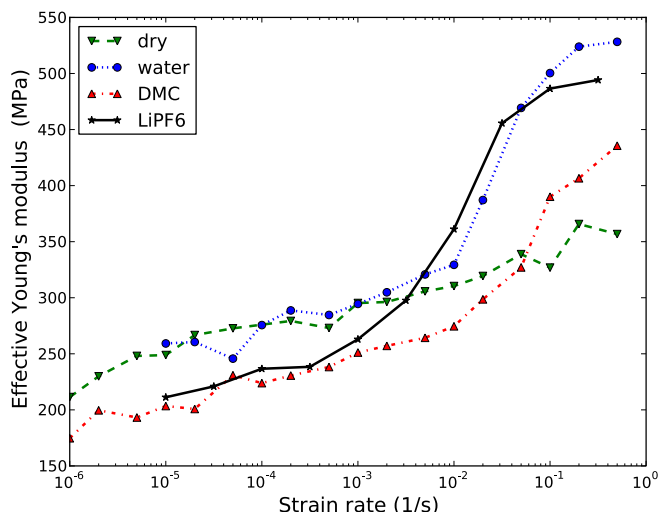
Figure 6. Effective Young's modulus of the dry separator, immersed in water, in DMC and in 1 M LiPF 6 solution in EC/DMC.
