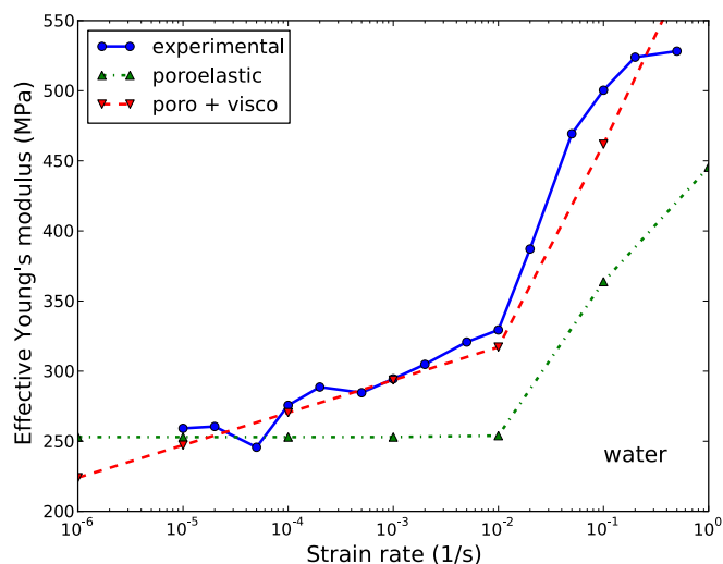
Figure 9. Effective Young's modulus of the separator immersed in water as a function of strain rate. The solid line gives the experimental data from 14 , the dash-dot line shows the calculations based on linear poroelastic behavior of the dry separator; and the dash line shows the calculations taking into account viscoelastic behavior of the dry separator when solving the equations of poroelasticity.
