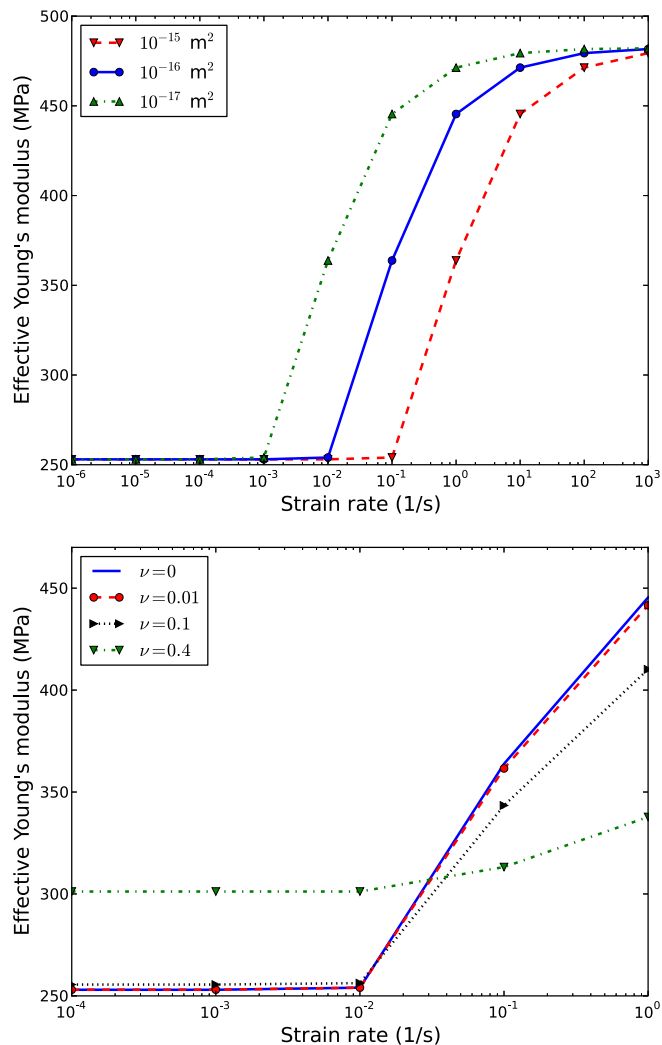
Figure 8. Effective Young's modulus calculated based on poroelasticity (top) for \nu = 0 and different values of permeability k (bottom) for k = 10^{-16} m ^2 and different values of Poisson's ratio \nu .
