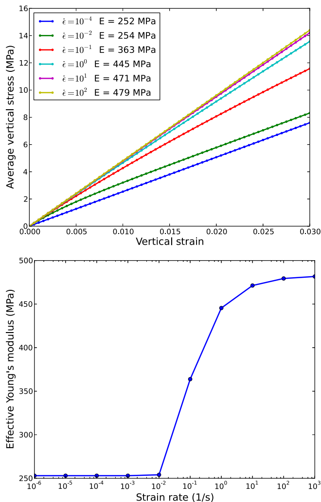
Figure 7. (top) Stress-strain curves calculated from finite-element simulations of vertical compression of porous separator at selected strain rates (bottom) Effective Young's modulus estimated from these stress-strain curves as a slope at 2% strain.
