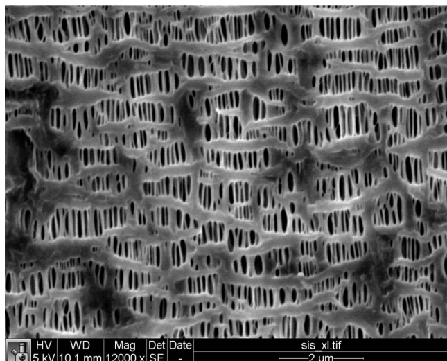
Figure 1. SEM image of the Celgard 3501 separator used in experiments in the plane perpendicular to the compression.
