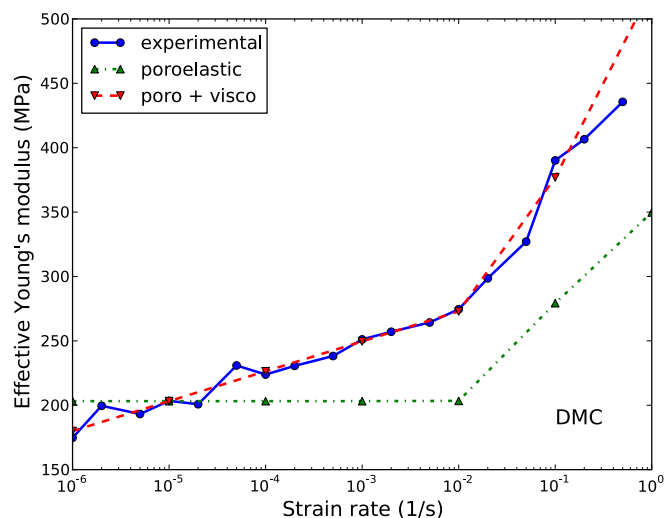
Figure 10. Effective Young's modulus of the separator immersed in DMC as a function of strain rate. Solid line represents the experimental data from 14 , dash-dot line shows the results of calculations based on linear poroelastic behavior of the dry separator; red line shows the results of calculations, which take into account viscoelastic behavior of the dry separator and softening of the separator in DMC when solving the equations of poroelasticity.
